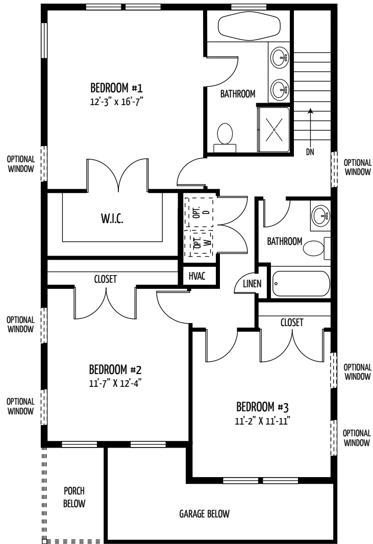
COOLIDGE OPTIONAL SECOND FLOOR
