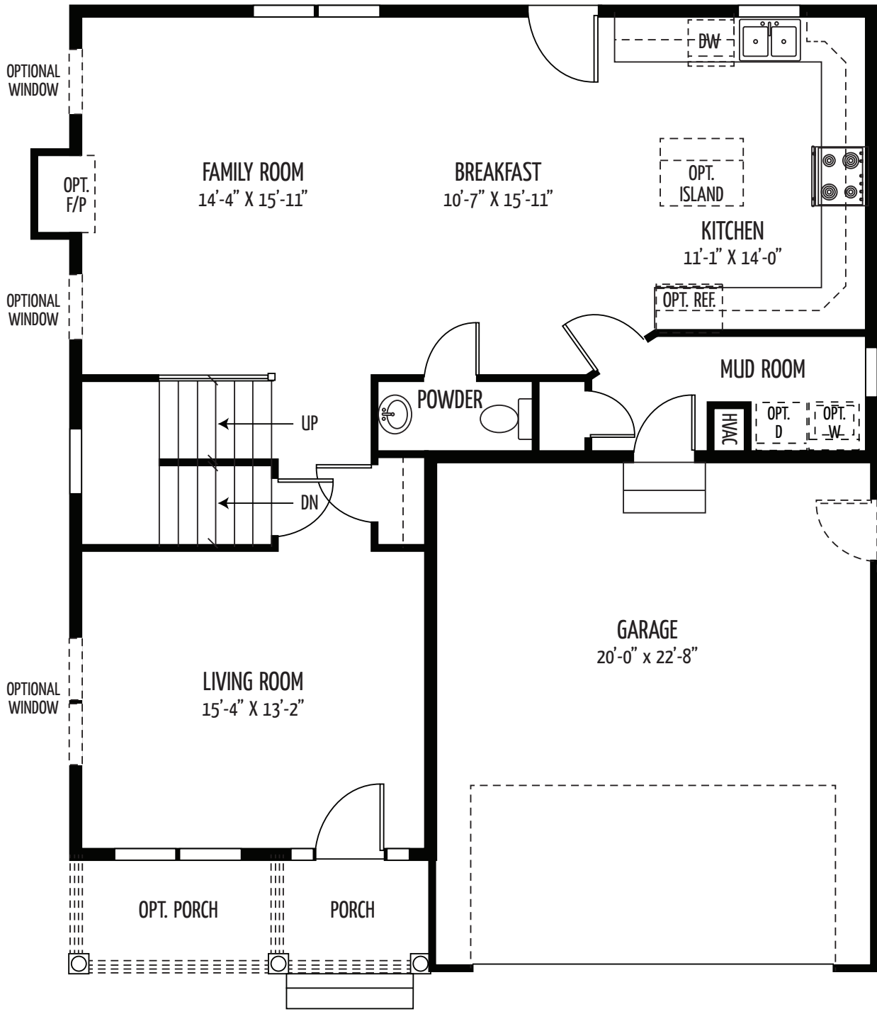
HARDING FIRST FLOOR
