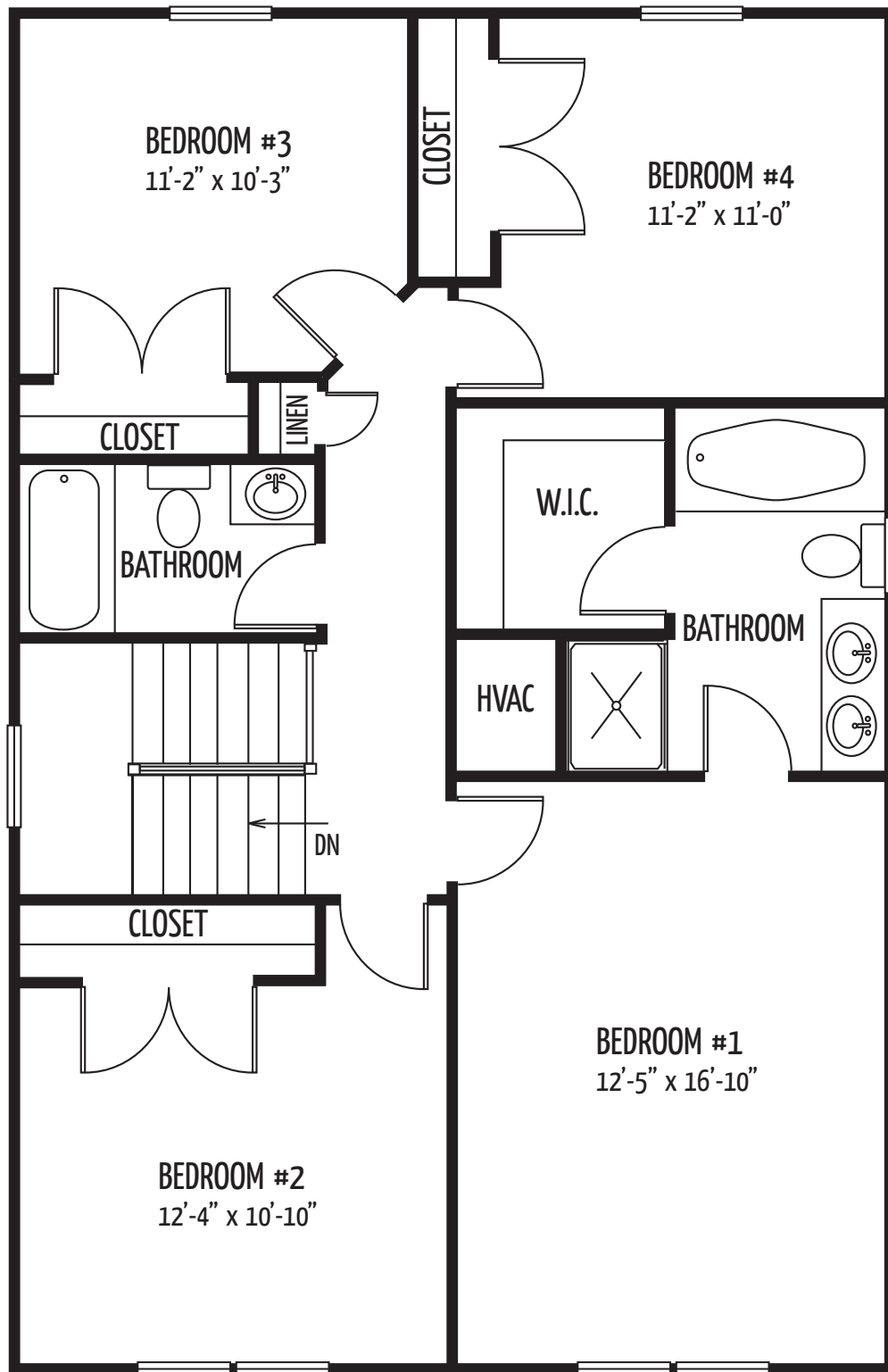
HARFORD OPTIONAL ALTERNATE SECOND FLOOR
