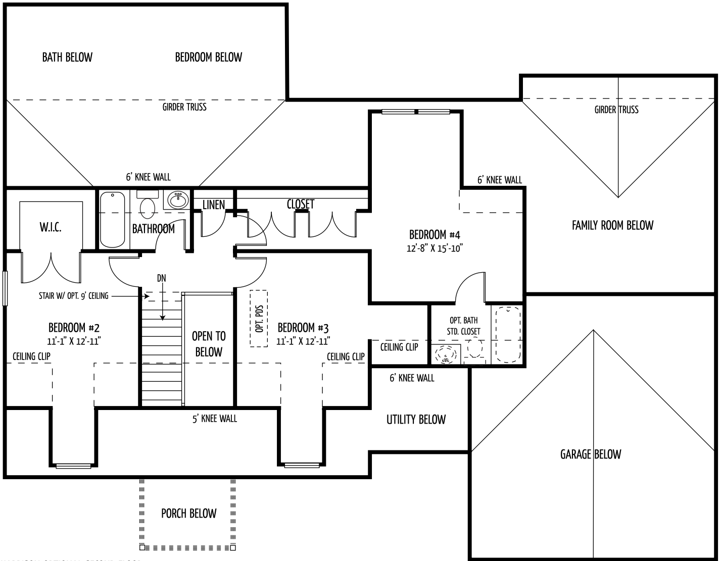
HARRISON OPTIONAL SECOND FLOOR
