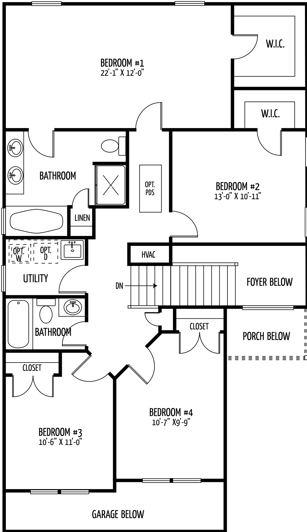
SEVERN SECOND FLOOR
