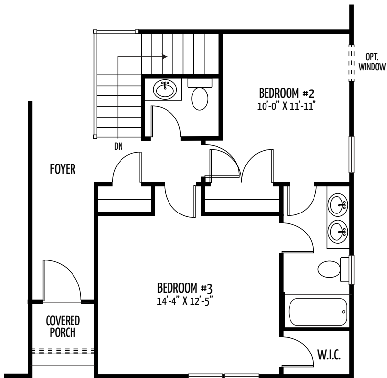
GEORGETOWN ELEVATION C/D - ALTERNATE PLAN
