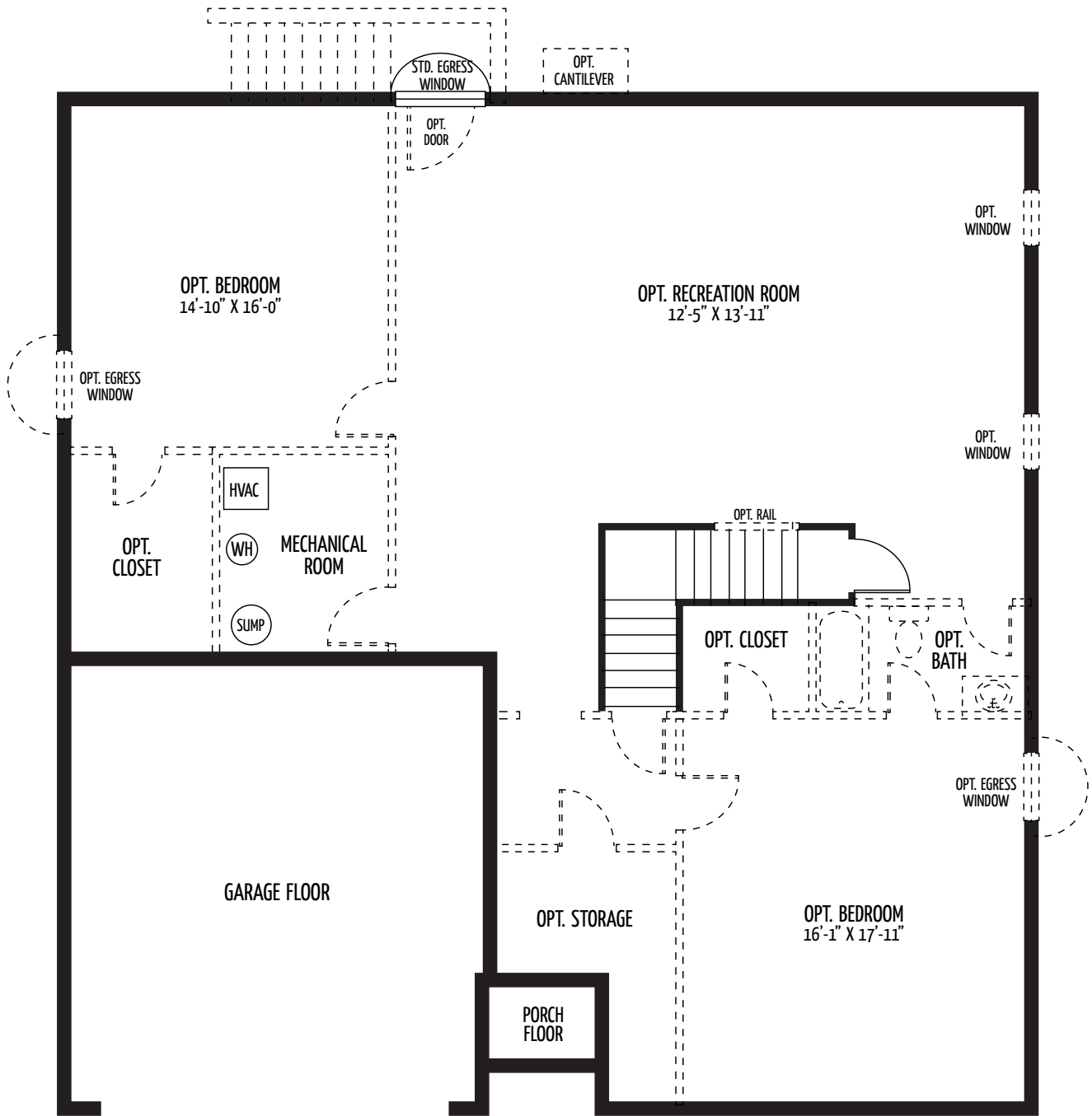
GEORGETOWN C/D BASEMENT
