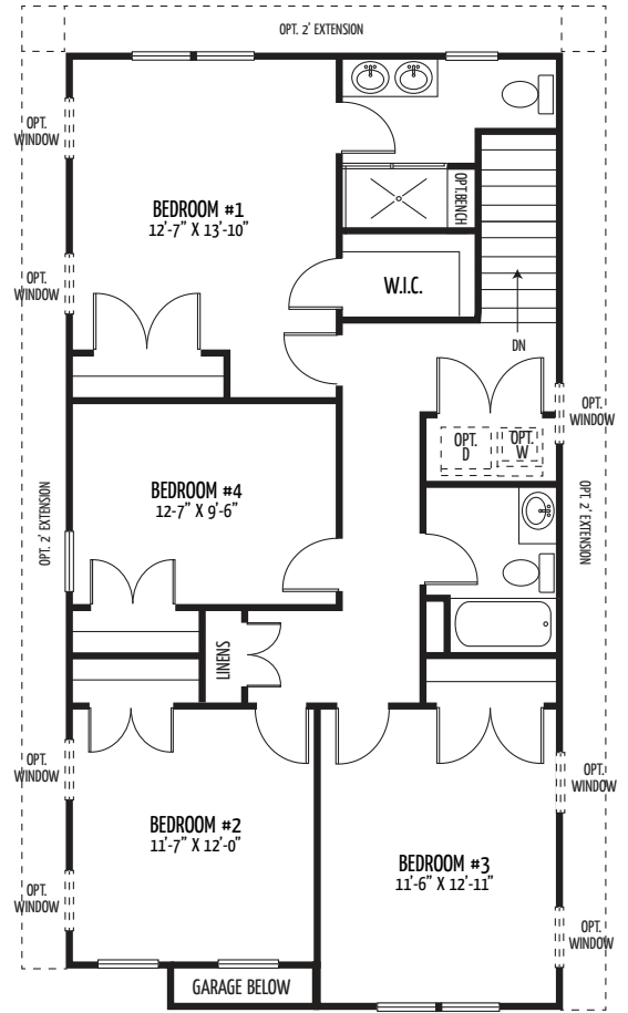
COOLIDGE ELEVATION C/D - SECOND FLOOR
