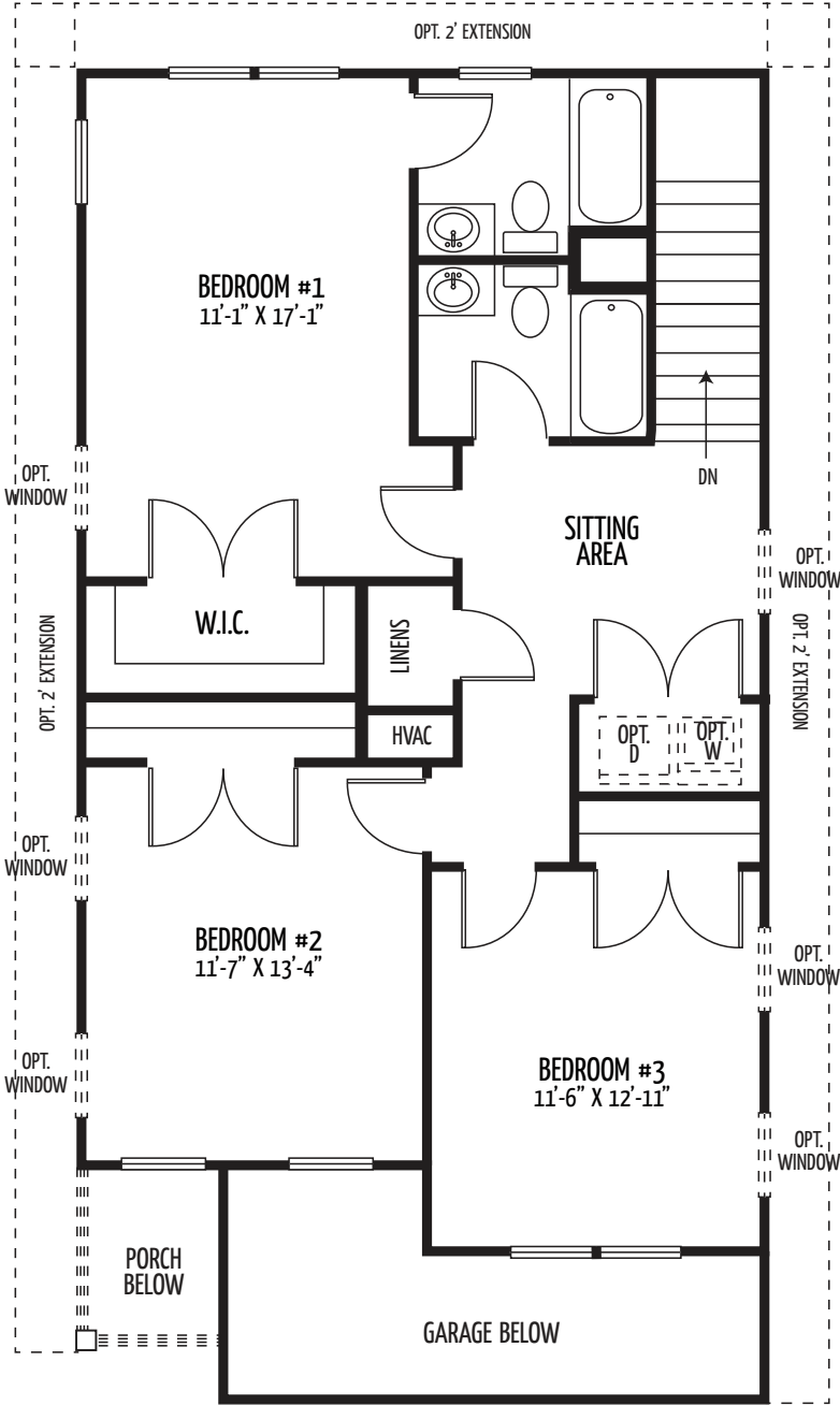
COOLIDGE - STANDARD SECOND FLOOR
