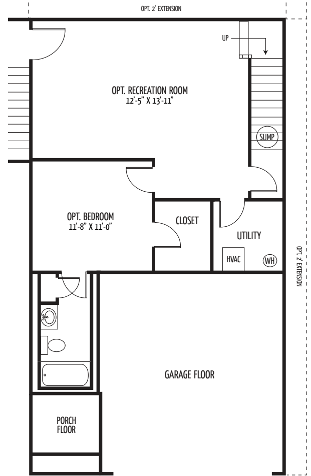
COOLIDGE - OPTIONAL BASEMENT (W/ LOWER LEVEL BED & BATH AND 2' LEFT SIDE EXTENSION)
