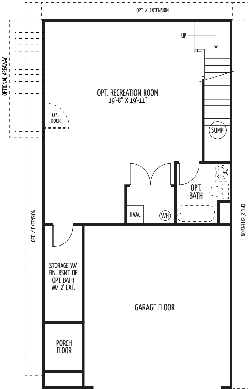
COOLIDGE - STANDARD BASEMENT
