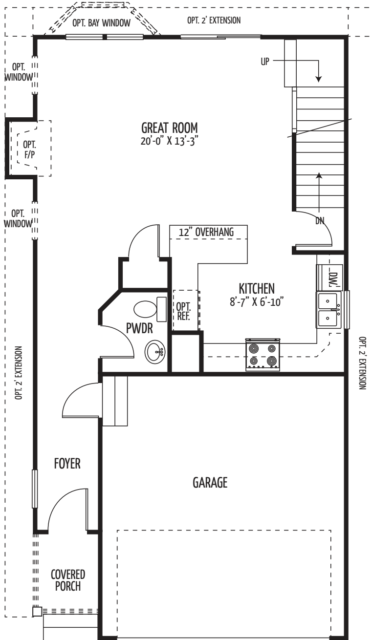
COOLIDGE - FIRST FLOOR
